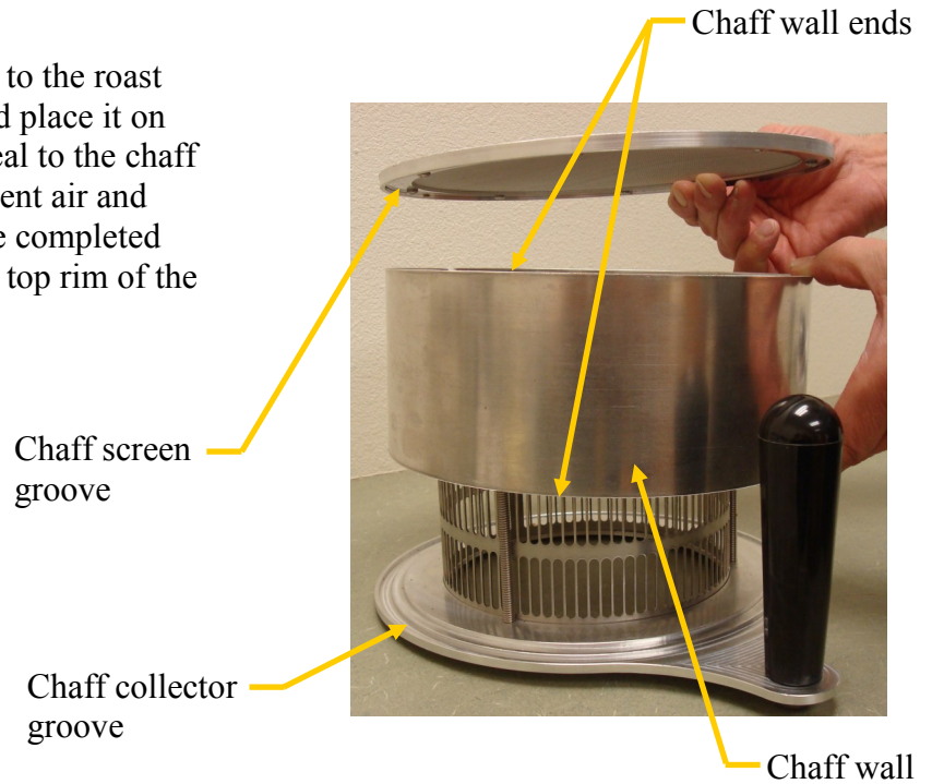
Completed roast chamber/chaff collector assembly.
