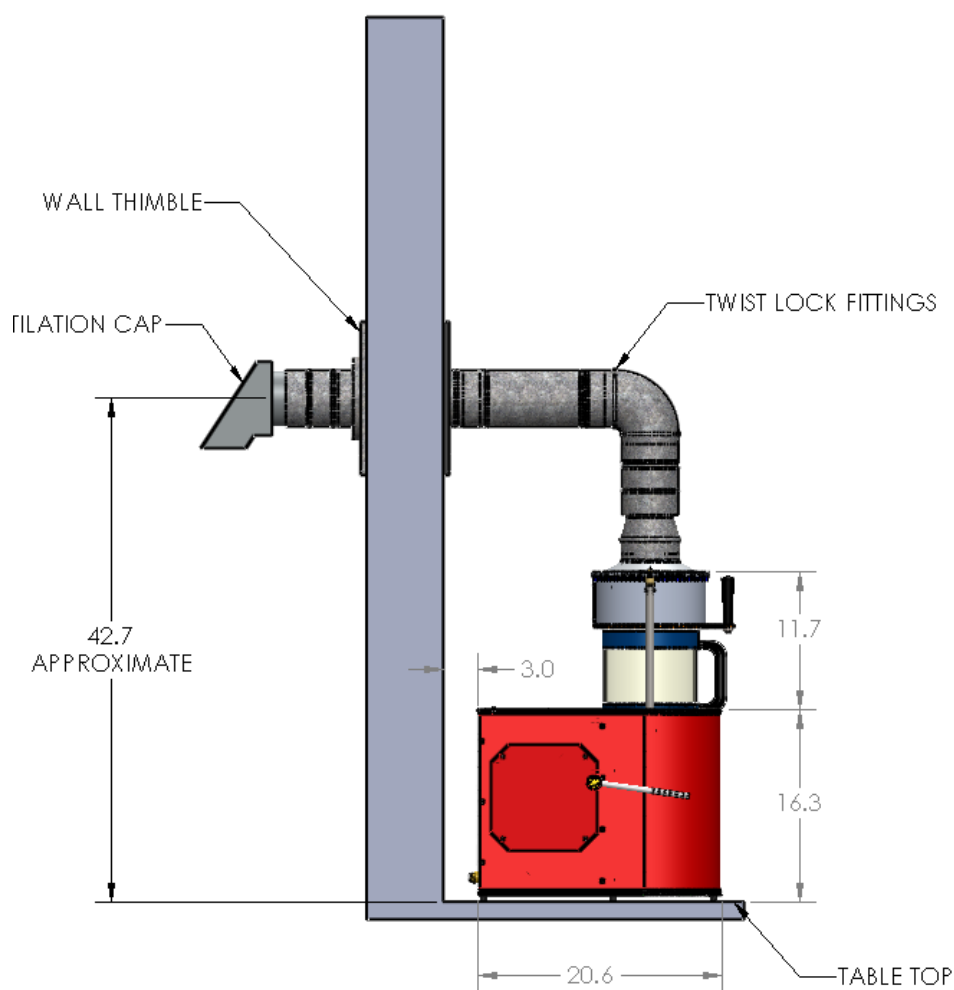
TYPICAL DIRECT VENT INSTALLATION SONOFRESCO VK-100 VENT KIT SHOWN ROASTER WIDTH APPROX. 13.5" WIDE
